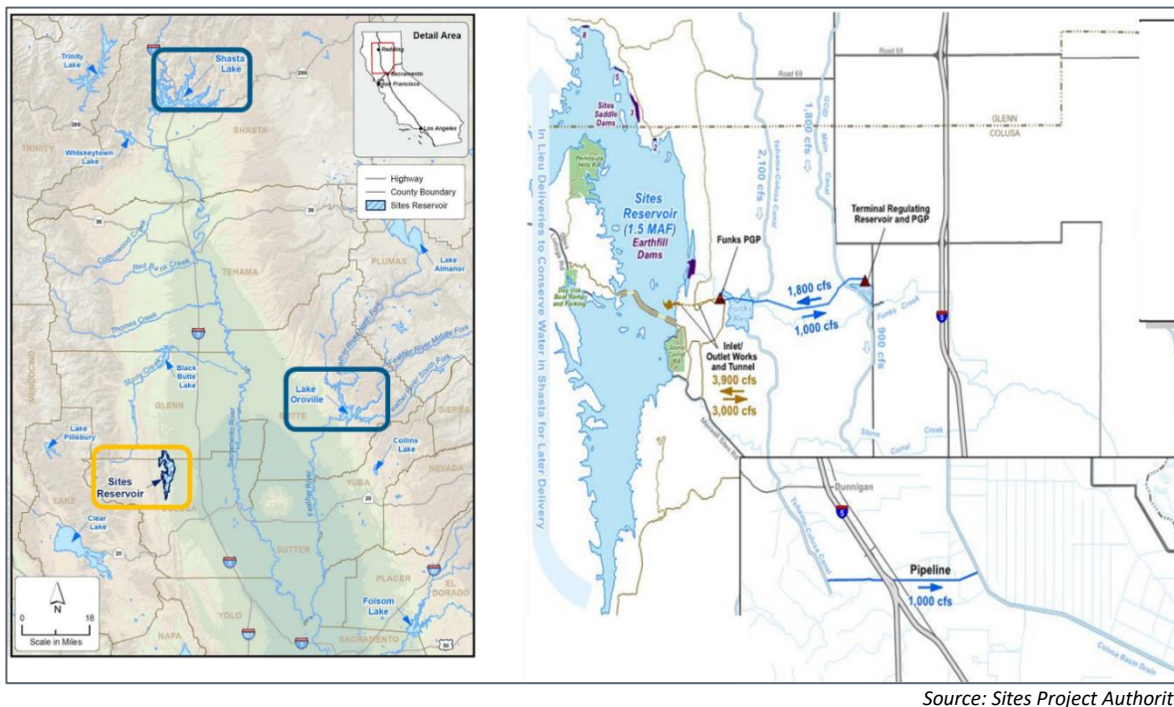
Figure 6-7. Sites Reservoir Project: Location and Facilities
