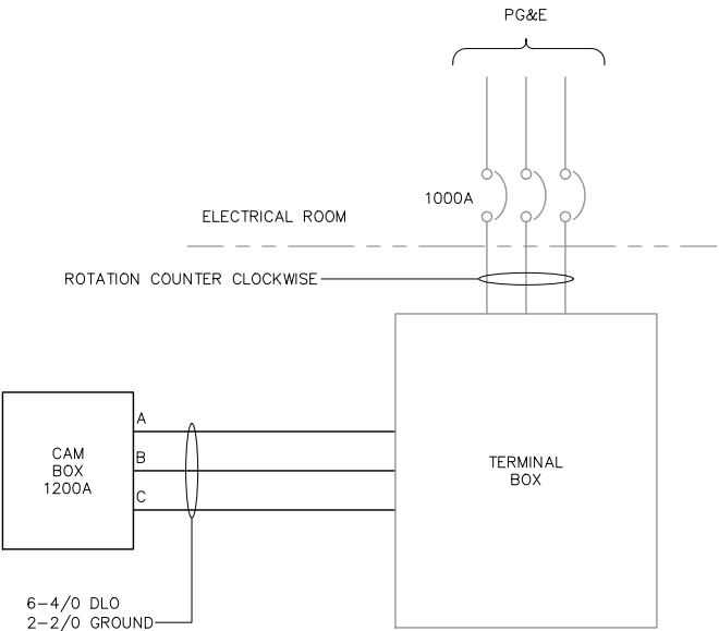
ELECTRICAL CONNECTION DETAIL NONE
