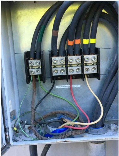
TRANSFER SWITCH
