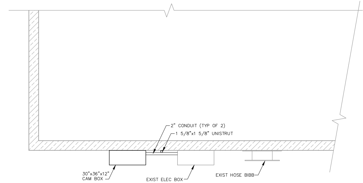
PLAN NONE
