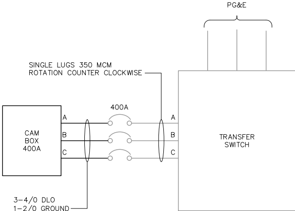
ELECTRICAL CONNECTION DETAIL NONE
