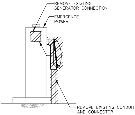
SECTION NONE
