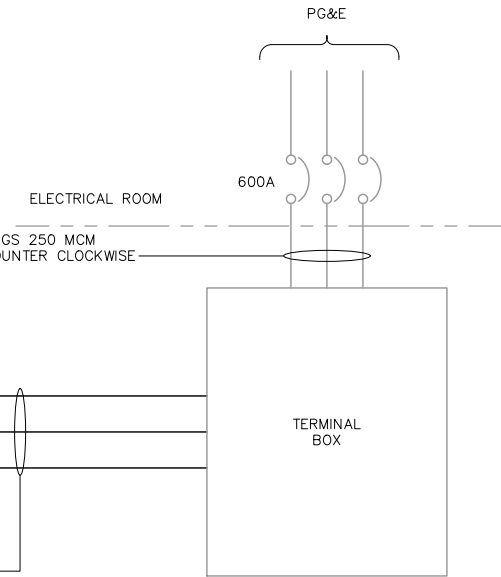
ELECTRICAL CONNECTION DETAIL NONE
